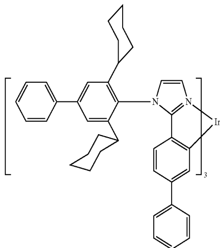
Compound 23
