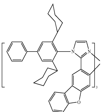
Compound 17
