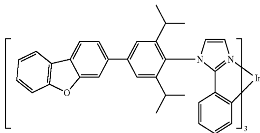
Compound 36
