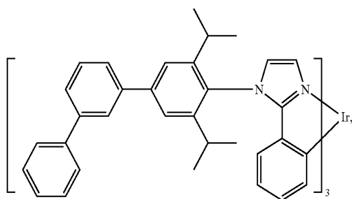
Compound 29
