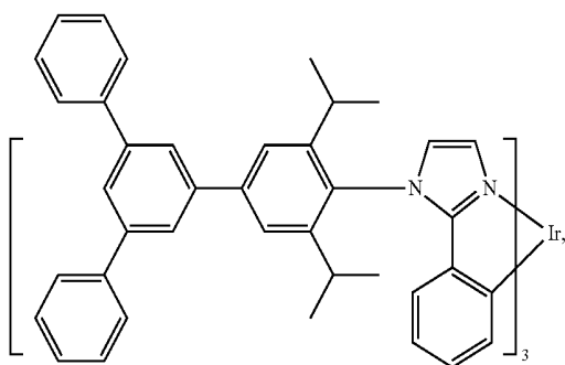
Compound 31
