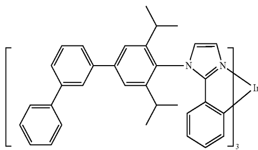
Compound 29
