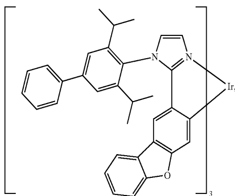
Compound 8
