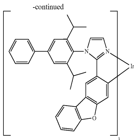
Compound 7
