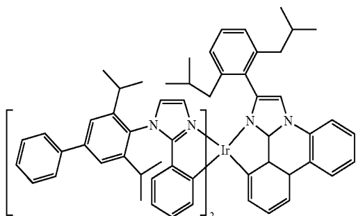
Compound 58
