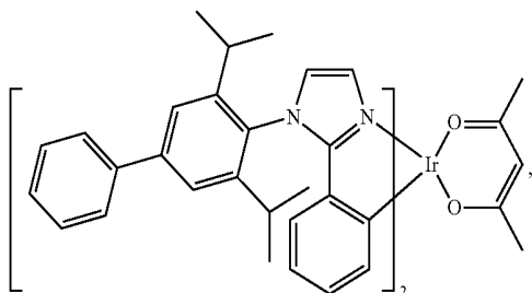
Compound 49
