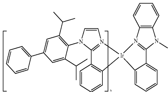
Compound 51
