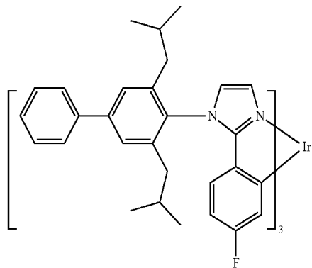
Compound 27
