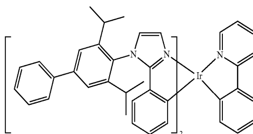
Compound 47
