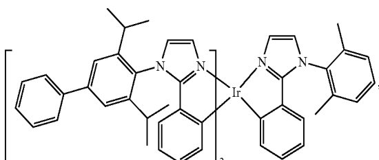
Compound 50
