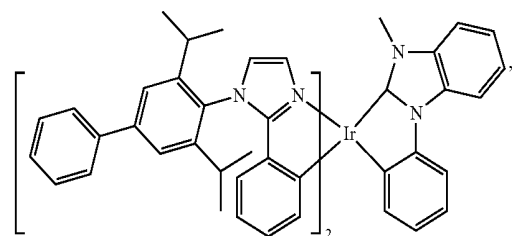
Compound 56
