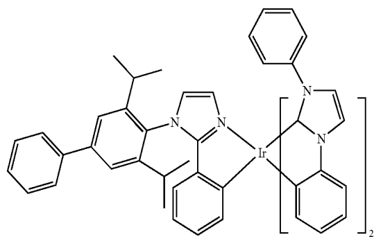
Compound 66
