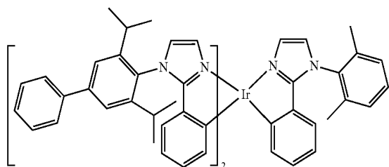
Compound 51
