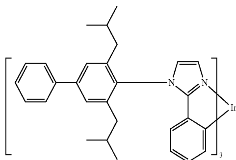
Compound 5
