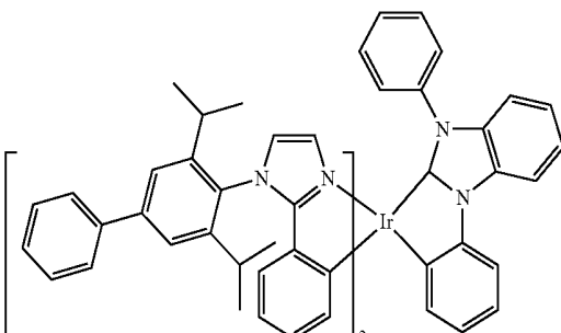
Compound 57
