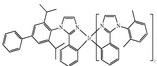
Compound 61
