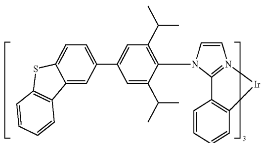
Compound 32
