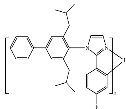
Compound 27
