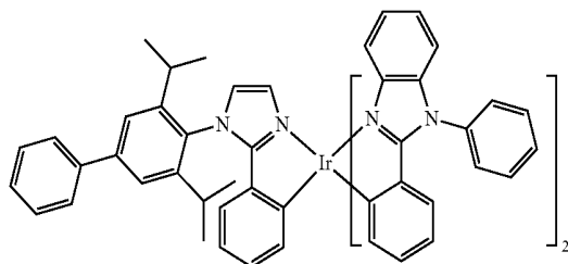
Compound 64
