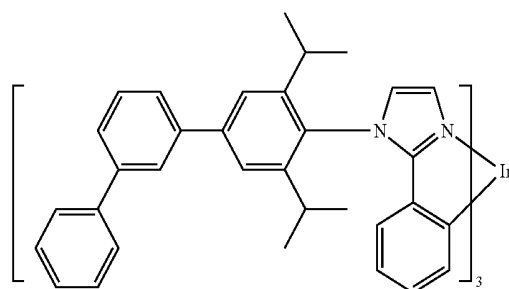
Compound 29
