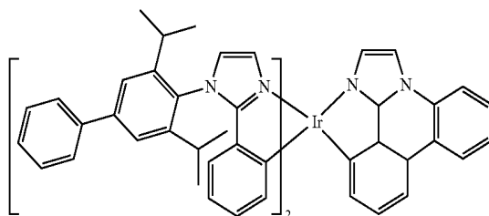
Compound 57
