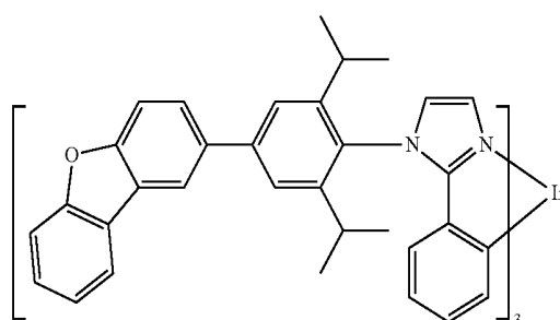
Compound 35
