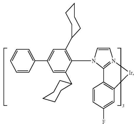
Compound 28
