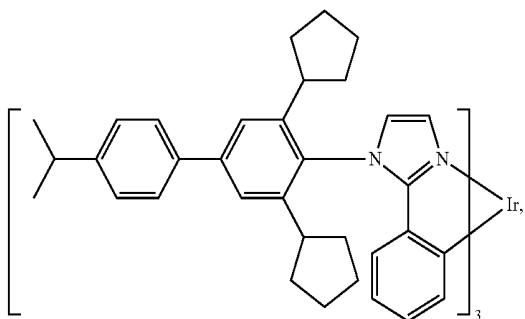
Compound 10
