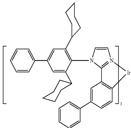
Compound 17
