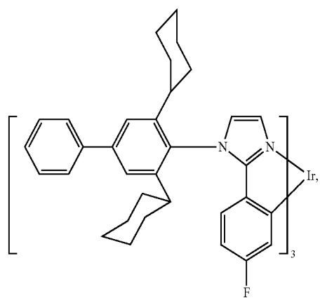
Compound 28
