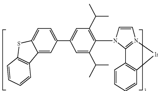
Compound 32
