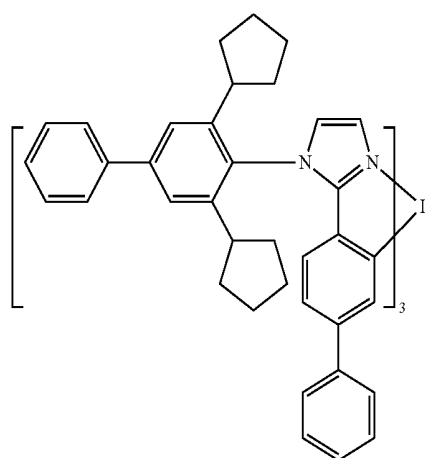
Compound 21
