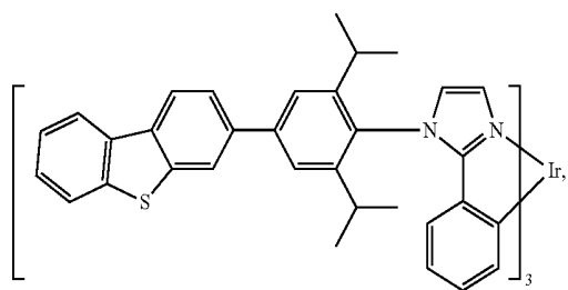
Compound 33
