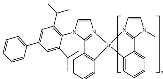
Compound 61
