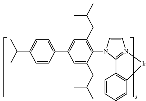
Compound 12
