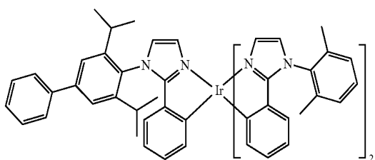
Compound 61
