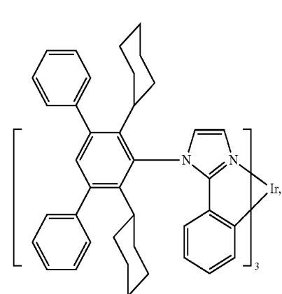
Compound 46
