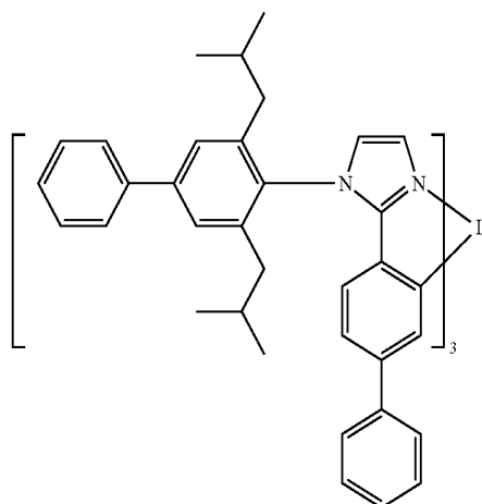
Compound 22
