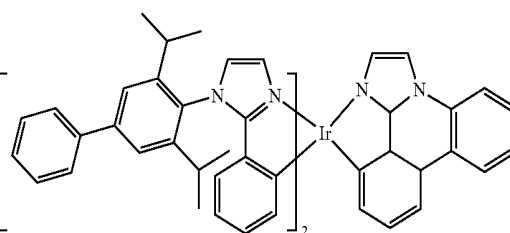
Compound 57
