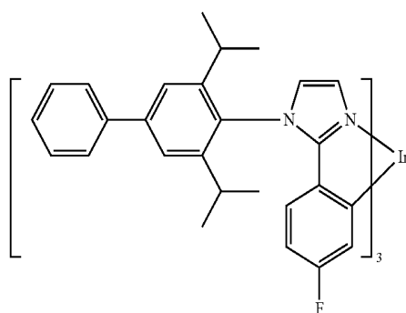
Compound 29
