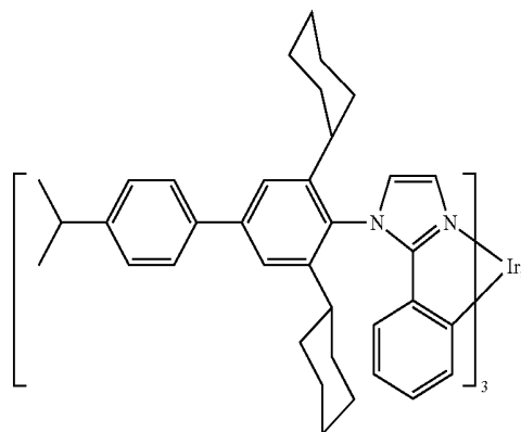
Compound 14
