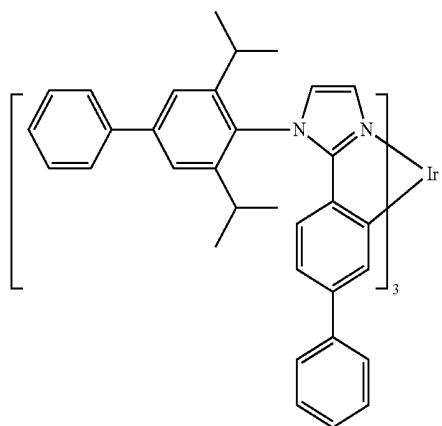
Compound 24
