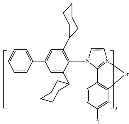
Compound 28
