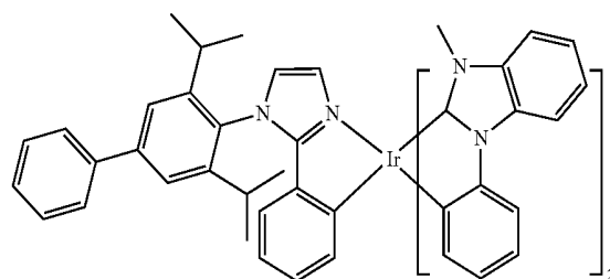
Compound 66
