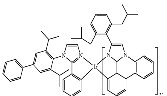
Compound 69
