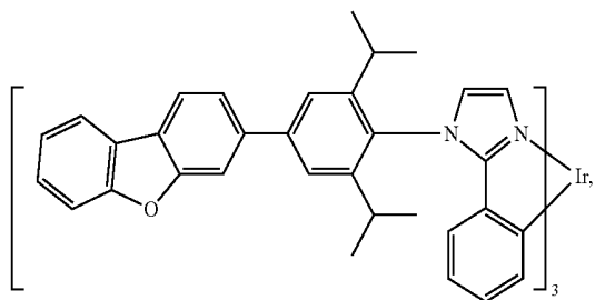
Compound 36
