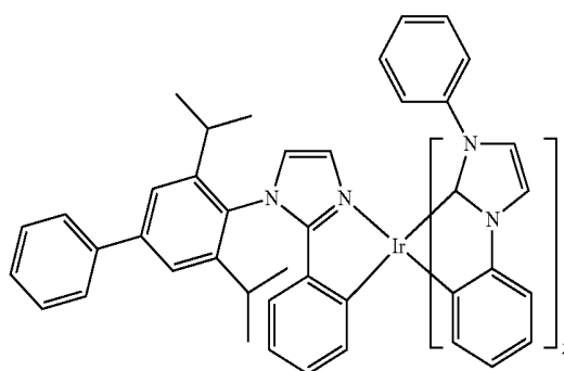
Compound 66
