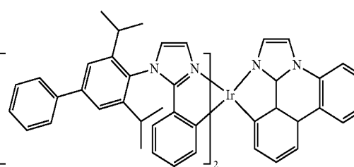
Compound 58
