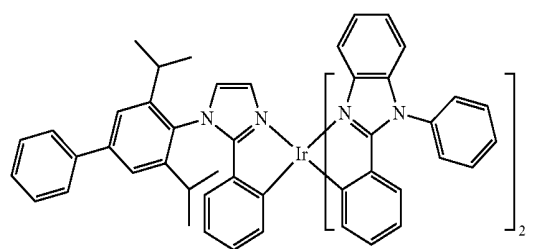
Compound 63
