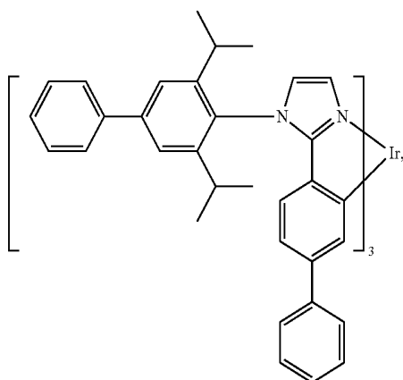
Compound 24
