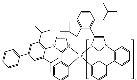
Compound 69
