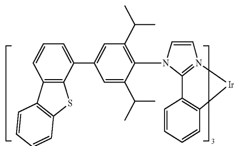
Compound 34
