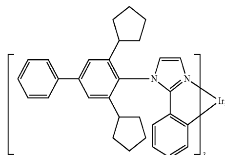
Compound 8
