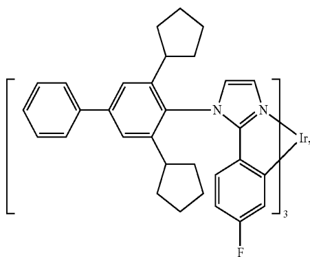
Compound 25
