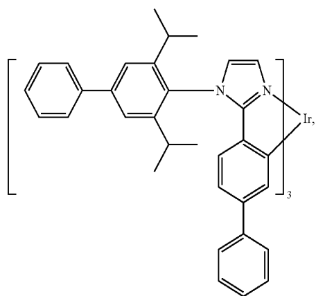
Compound 24
