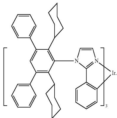
Compound 42
