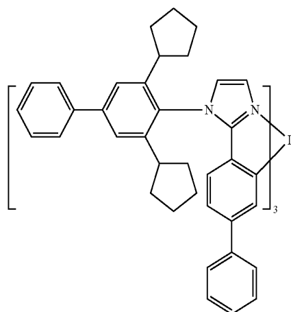
Compound 21
