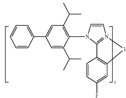
Compound 28
