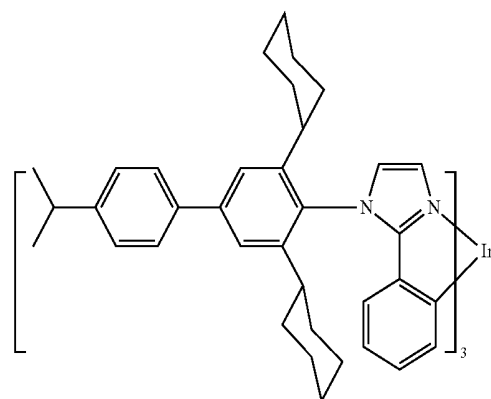
Compound 14
