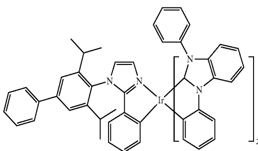
Compound 67
