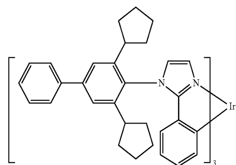
Compound 8
