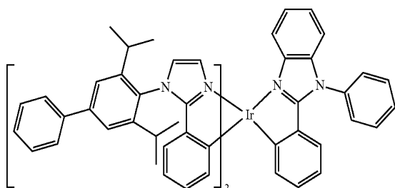
Compound 52
