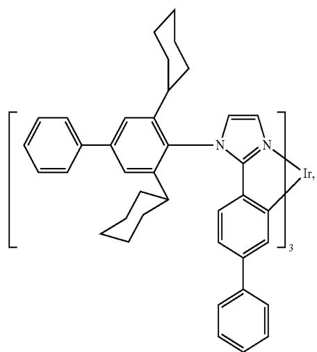
Compound 23
