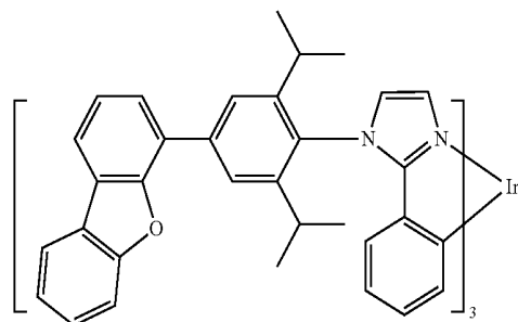
Compound 37
