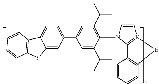
Compound 33
