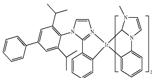
Compound 65
