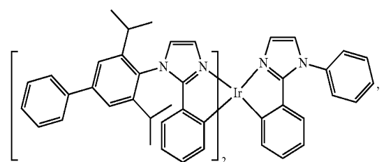
Compound 52
