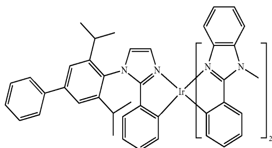
Compound 62
