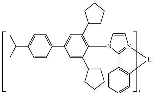
Compound 11
