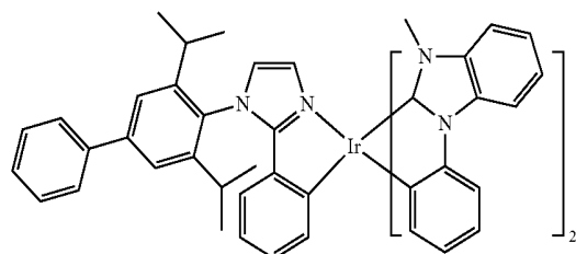
Compound 66
