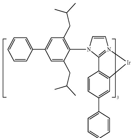
Compound 22
