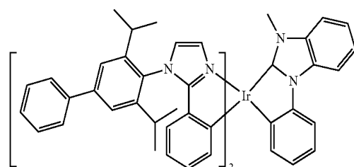
Compound 56
