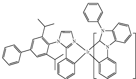
Compound 67
