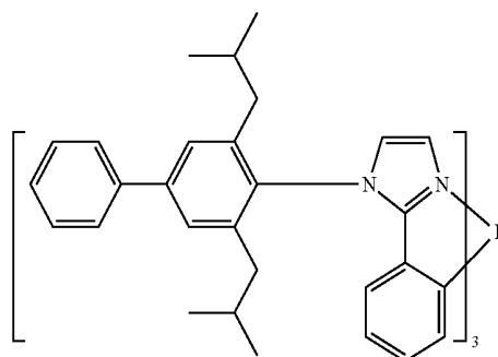
Compound 5
