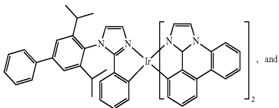
Compound 69
