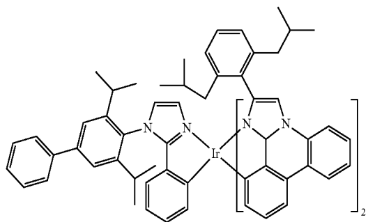
Compound 69
