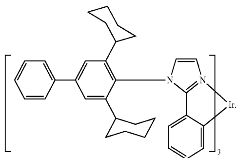
Compound 3
