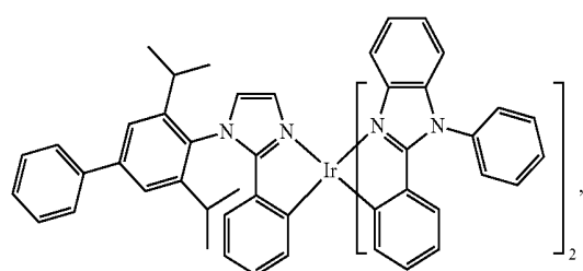
Compound 63
