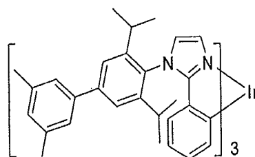
Compound 2
