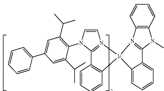
Compound 51
