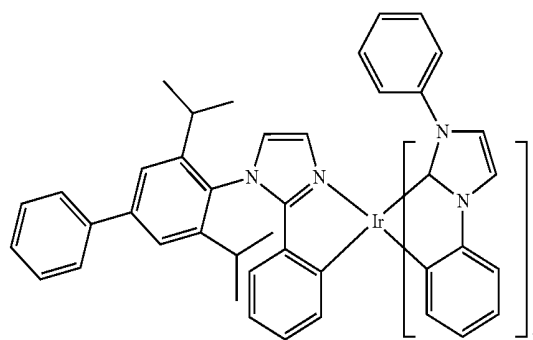
Compound 65
