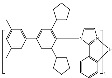
Compound 9
