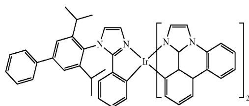
Compound 68
