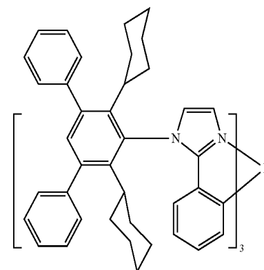
Compound 42
