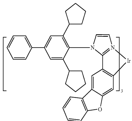
Compound 18
