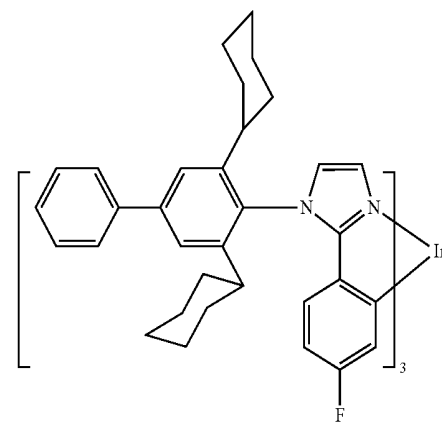
Compound 28
