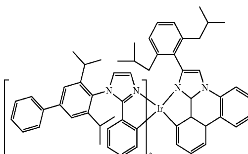
Compound 58
