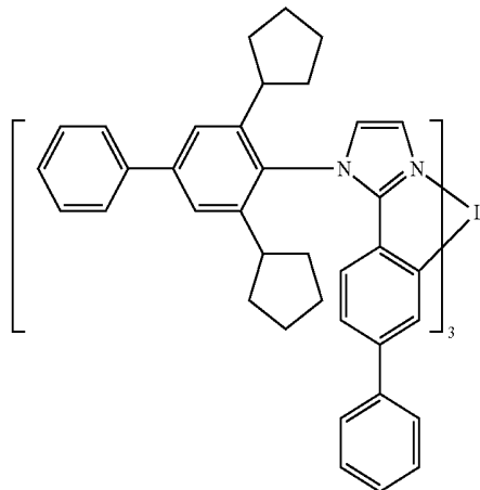
Compound 21
