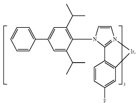
Compound 28
