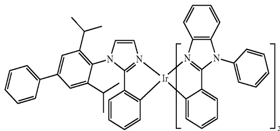
Compound 64
