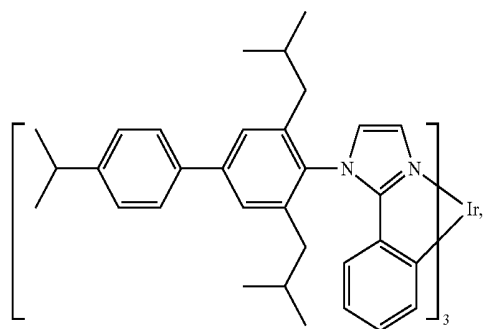
Compound 12
